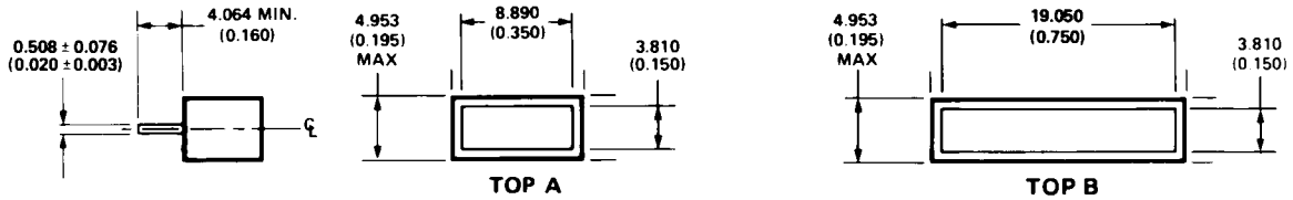
END VIEW A, B
