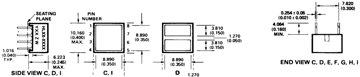
SIDE VIEW C, D, I
