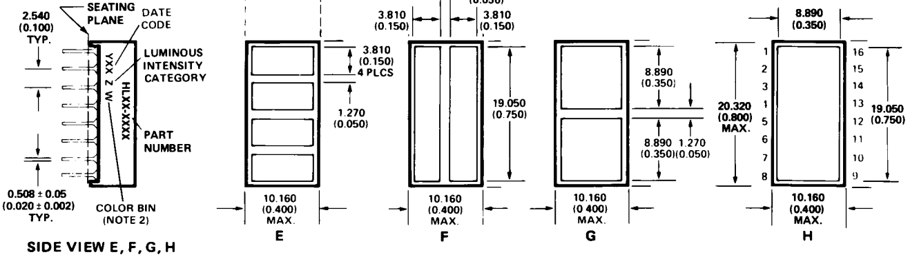
SIDE VIEW E, F, G, H
